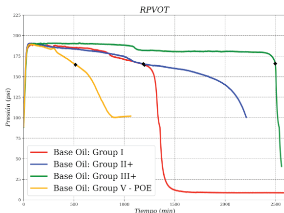
Figure 2: RPVOT curves for different base oil formulations.
