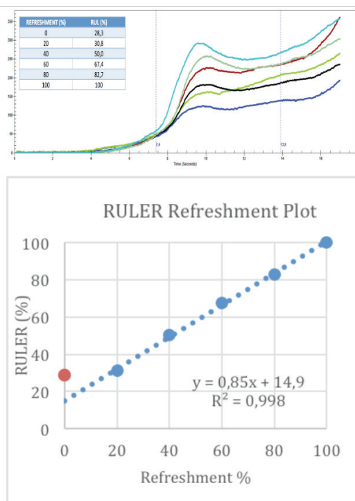
Figure 3. RULER can be quantified by extrapolation in degraded samples.
